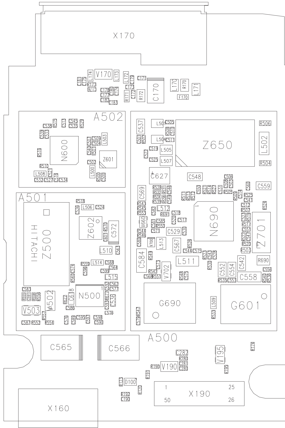
Parts Placement Diagram of BS2 _09
